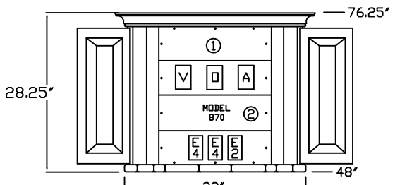
FRONT VIEW WITH DOORS OPEN
